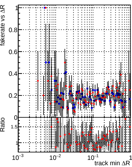
Fake rate vs \Delta R (track, jet) DQM_TTbarTEST DQM_CKF_TTbar
