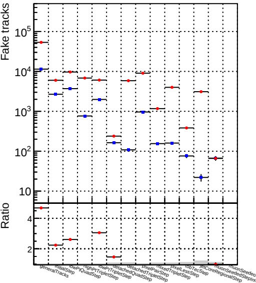
Number —●— DQM_CKF_TTbar
