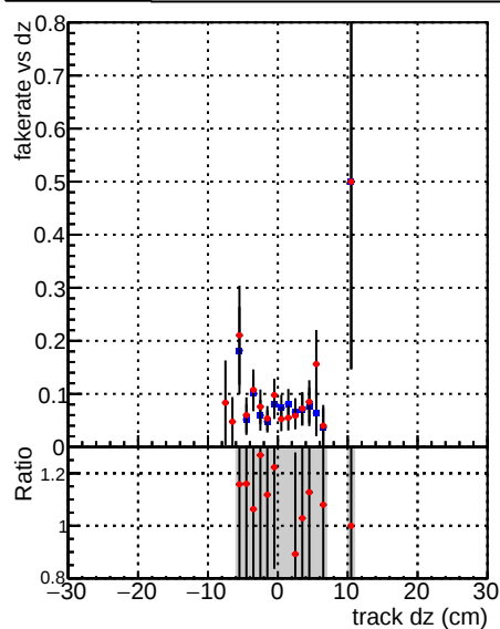
—•— DQM_TTbarTEST —•— DQM_CKF_TTbar
