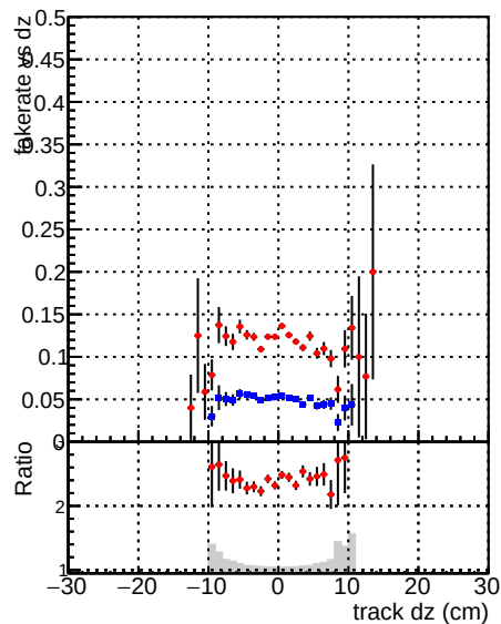
—■— DQM_TTbarTEST —●— DQM_CKF_TTbar
