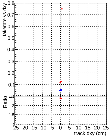
—■— DQM_TTbarTEST —●— DQM_CKF_TTbar
