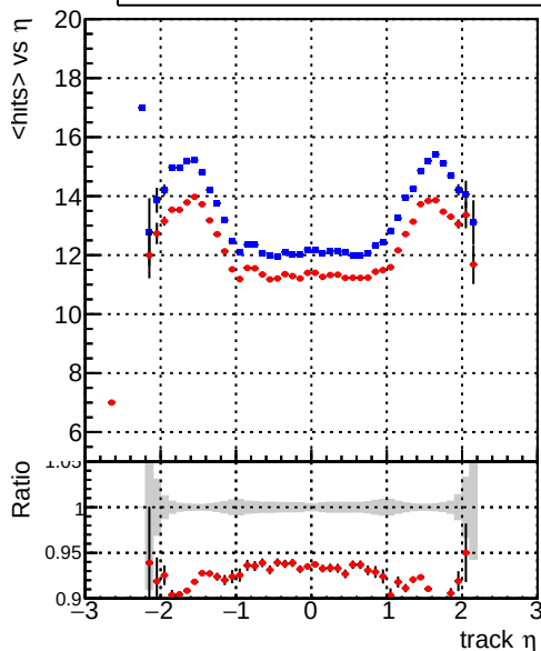
— DQM_TTbarTEST — DQM_CKF_TTbar mean hits vs \eta
