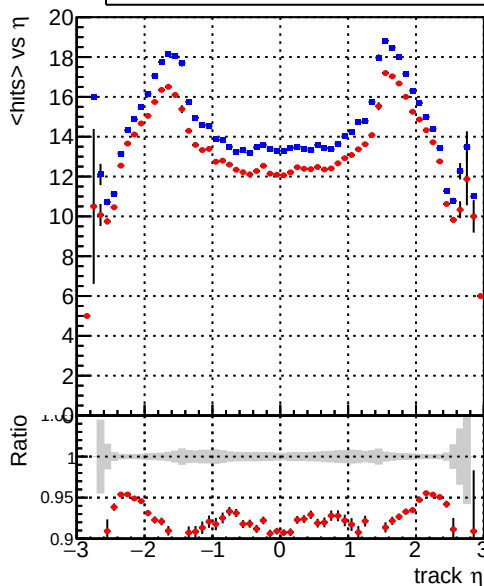
mean hits vs \eta — DQM_TTbarTEST — DQM_CKF_TTbar
