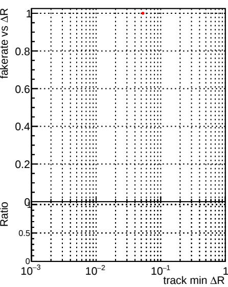
Fake rate vs \Delta R(\text{track, jet}) Legend: DQM_TTbarTEST (grey line with blue dots) DQM_mkFitTTbarTEST (black line with red dots)
