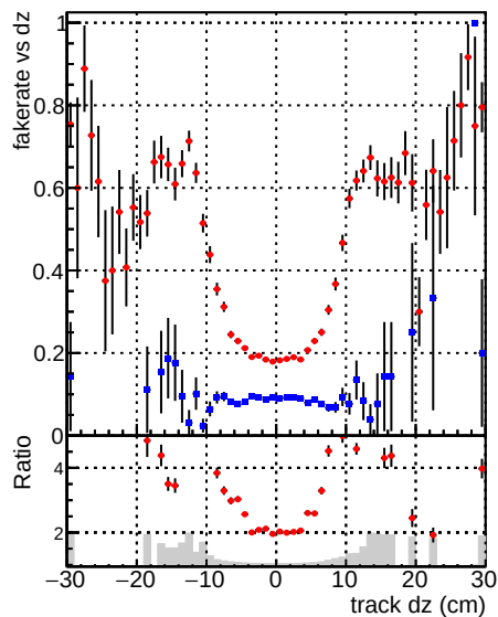
—●— DQM_TTbarTEST —●— DQM_mkFitTTbarTEST
