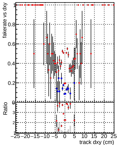
—●— DQM_TTbarTEST —●— DQM_mkFitTTbarTEST
