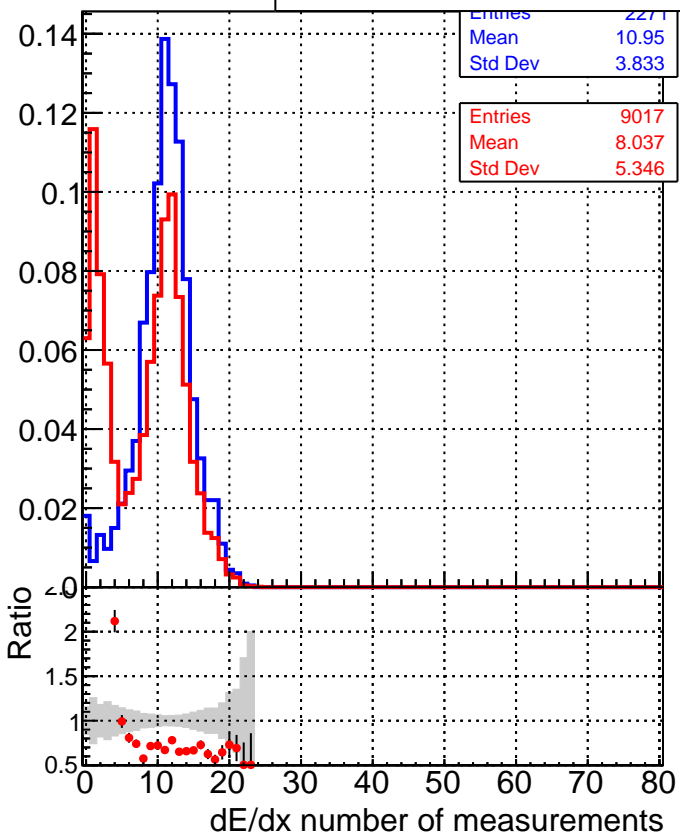
—■— DQM_TTbarTEST —●— DQM_mkFitTTbarTEST
