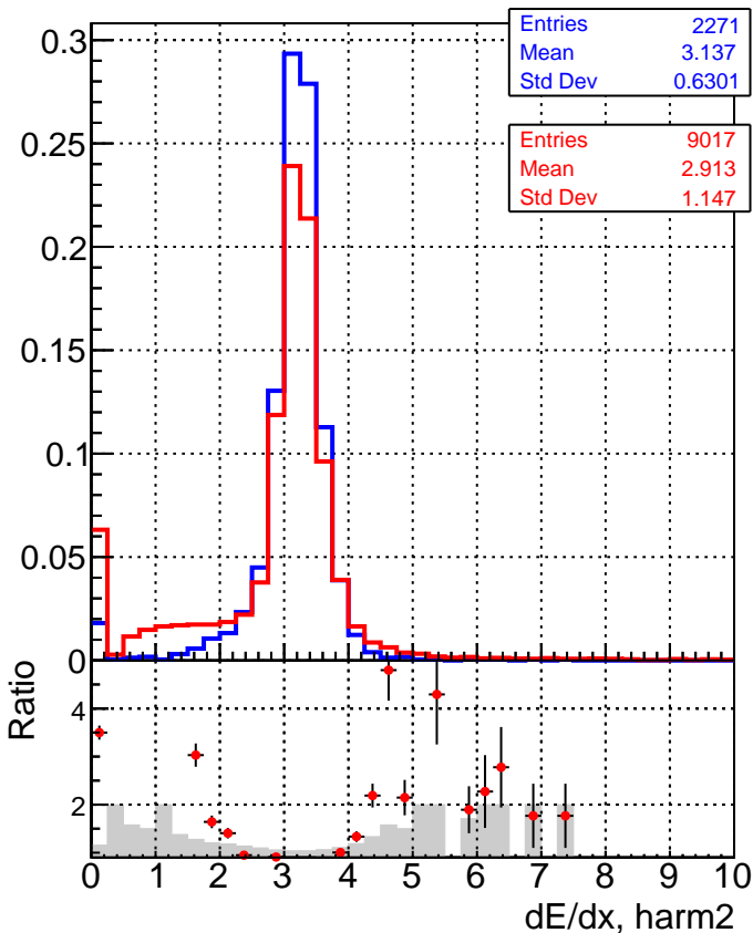
—■— DQM_TTbarTEST —●— DQM_mkFitTTbarTEST
