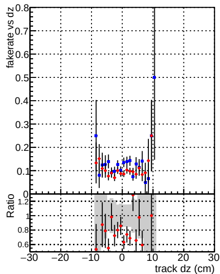
—●— DQM_TTbarTEST —●— DQM_mkFitTTbarTEST
