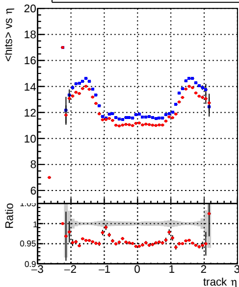
DQM_TTbarTEST mean hits DQM_mkFitTTbarTEST
