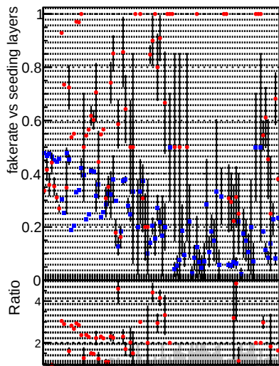
Fake rate vs. —♦— DQM_TTbarTEST —♦— DQM_mkFitTTbarTEST
