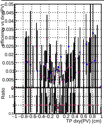
Efficiency vs Dxy(PV) (cm) DOM_mkFit_TT_retrain DOM_mkFit_TT_NEWdefault_specPless1 DOM_mkFit_TT_NEWdefault_specPless2 DOM_mkFit_TT_NEWdefault_specPless3 DOM_mkFit_TT_NEWdefault_specPless4
