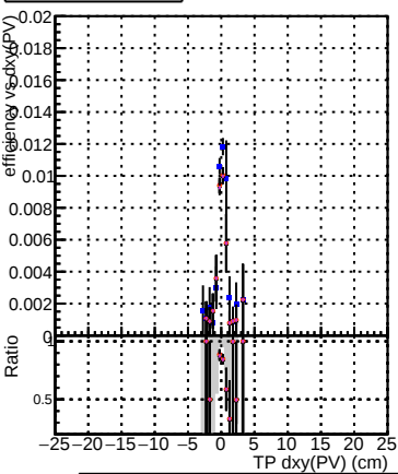
Efficiency vs Dxy(PV) (cm) DOM_mkFit_TT_retrain DOM_mkFit_TT_NEWdefault_specPless1 DOM_mkFit_TT_NEWdefault_specPless2 DOM_mkFit_TT_NEWdefault_specPless3 DOM_mkFit_TT_NEWdefault_specPless4
