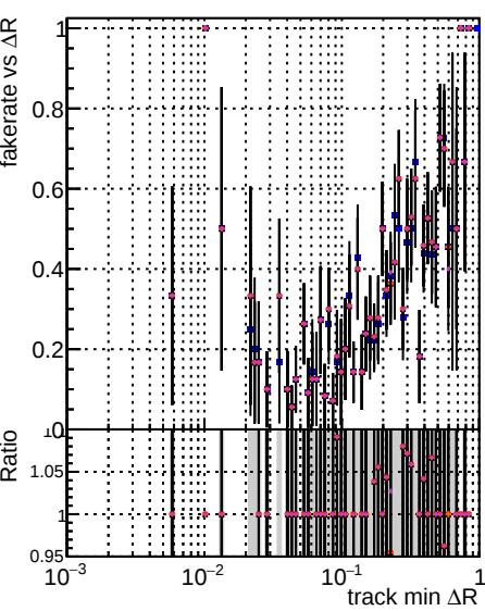
Fake rate vs \Delta R(\text{track, jet}) Legend: DOM (blue), mktFit (orange), TT retrain (green), Newdata (red), Newdata (purple), specCB (black), Less1 (grey), Less2 (light grey), Less3 (very light grey), Less4 (white).
