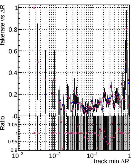
Fake rate vs \Delta R(\text{track, jet}) Legend: DOM (black), mktFit (blue), mktFit+retrain (red), Newdata (green), Newdata+retrain (purple), specCBLess1 (cyan), specCBLess2 (magenta), specCBLess3 (yellow), specCBLess4 (orange).
