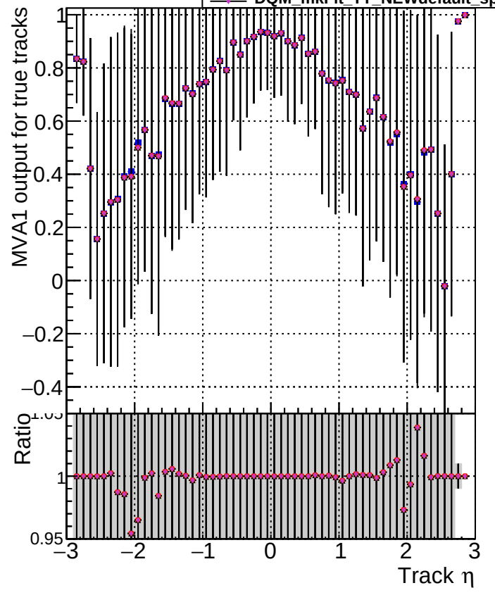
MVA1 of associated tracks (recoToSim) vs. track \eta Legend: DOM mkFit TT retrain (blue square) DOM mkFit TT NEWdefault specPless1 (red circle) DOM mkFit TT NEWdefault specPless2 (black triangle) DOM mkFit TT NEWdefault specPless3 (orange diamond) DOM mkFit TT NEWdefault specPless4 (purple star)
