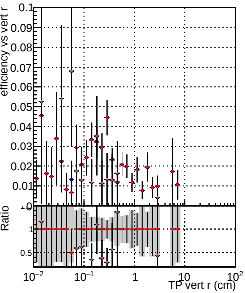
Efficiency vs vertpos Legend: DOM mkFit TT (eff) (blue line) DOM mkFit TT (NEWdefault specPLess1) (red line) DOM mkFit TT (NEWdefault specPLess2) (green line) DOM mkFit TT (NEWdefault specPLess3) (purple line) DOM mkFit TT (NEWdefault specPLess4) (pink line)
