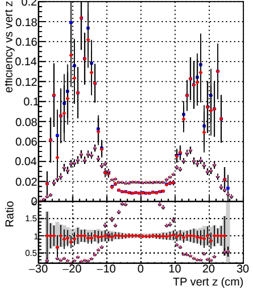
Efficiency vs. TP vert z (cm) DOM mkFit TT NEWdefault specPless1 DOM mkFit TT NEWdefault specPless2 DOM mkFit TT NEWdefault specPless3 DOM mkFit TT NEWdefault specPless4
