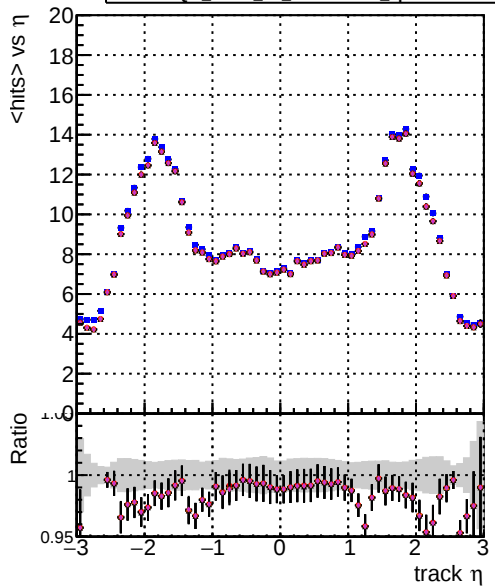
mean hits DOM mkFit TT (tdrw) DOM mkFit TT NEWdefault specPless1 DOM mkFit TT NEWdefault specPless2 DOM mkFit TT NEWdefault specPless3 DOM mkFit TT NEWdefault specPless4
