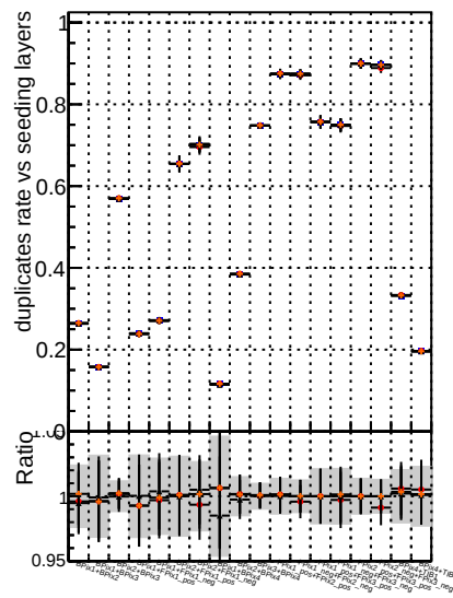
Match-CUT2 h-CUT2
