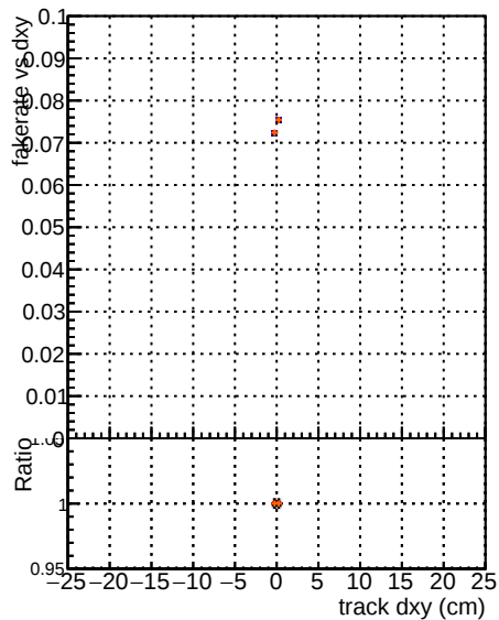
Legend for Fake rate vs d, Duplicates rate vs dz, and Pileup rate vs dz plots: — DOM mktFit TTXoriginal — DOM mktFit TTXWMS-genMatch-CUT2 — DOM mktFit TTXWMS-genMatch-CUT2
