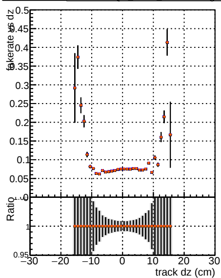
Legend for Fake rate vs d, Duplicates rate vs dz, and Pileup rate vs dz plots: — DOM mktFit TTXoriginal — DOM mktFit TTXWMS-genMatch-CUT2 — DOM mktFit TTXWMS-genMatch-CUT2
