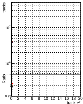
N of reco track vs. \chi^2 for various models and cuts
