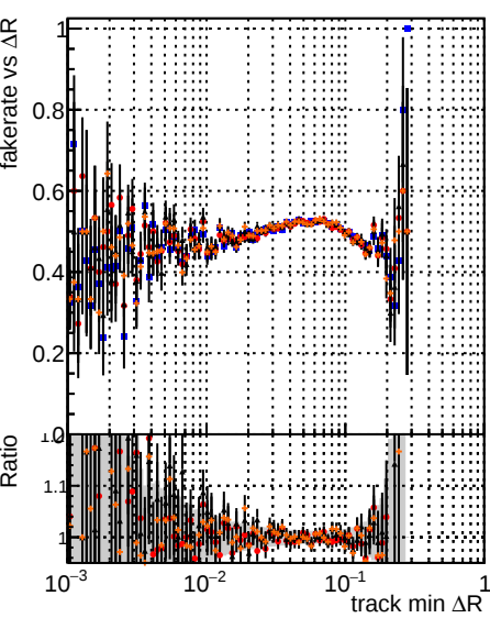
Fake rate vs \Delta R(\text{track, jet}) DOM mkFit T-Original T-NEWMS-genMatch-CUT2 DOM mkFit T-Original T-NEWMS-genMatch-CUT2-10% DOM mkFit T-Original T-NEWMS-genMatch-CUT2
