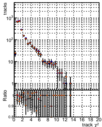
N of reco track vs. \chi^2 for BGM, mFit, TtoSim, genMatch-CUT2, mFit, TtoSim, genMatch-CUT2, mFit, TtoSim, genMatch-CUT2
