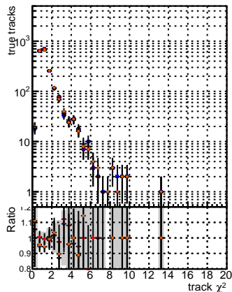
N of reco track vs. \chi^2 for BGM, mFit, TtoSim, genMatch-CUT2, mFit, TtoSim, genMatch-CUT2, mFit, TtoSim, genMatch-CUT2
