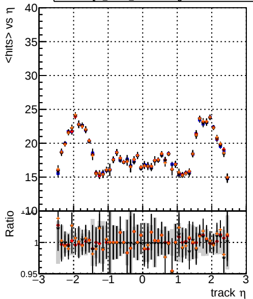
mean hit DQM_mkFit_TToriginal DQM_mkFit_TTNEWnoMS-genMatch-CUT2 DQM_mkFit_TToriginal-106 DQM_mkFit_TTNEWMS-genMatch-CUT2
