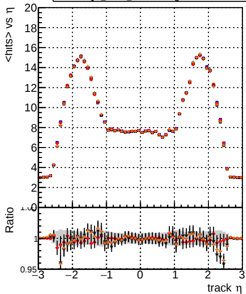
Legend: — DQM_mkFit_TToriginal — DQM_mkFit_TTNEWnoMS-genMatch-CUT2 — DQM_mkFit_TToriginal-106 — DQM_mkFit_TTNEWMS-genMatch-CUT2 mean hit
