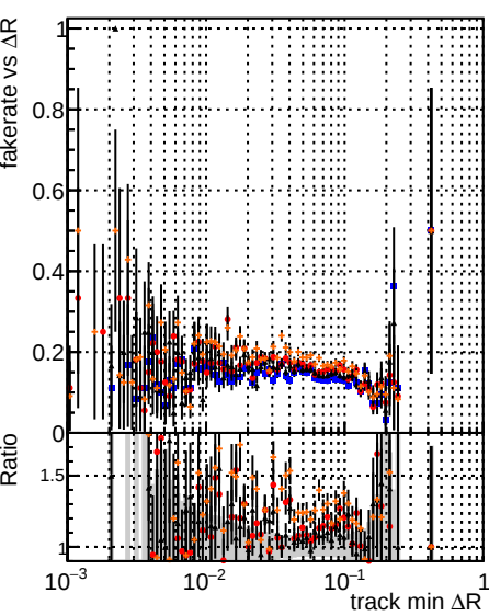
Fake rate vs \Delta R(\text{track, jet}) DOM mktFit T-Original DOM mktFit T-NEWMS-genMatch-CUT2 DOM mktFit T-NEWMS-genMatch-CUT2-10% DOM mktFit T-NEWMS-genMatch-CUT2
