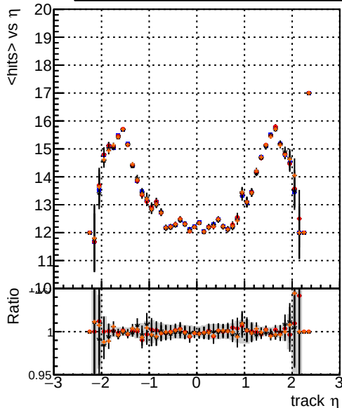
mean hits DQM_mkFit_TToriginal DQM_mkFit_TTNEWnoMS-genMatch-CUT2 DQM_mkFit_TToriginal-106 DQM_mkFit_TTNEWMS-genMatch-CUT2
