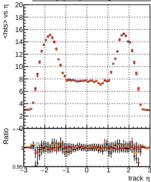
mean hit DOM_mkFit_TToriginal DOM_mkFit_TTNEWnoMS-genMatch-CUT2 DOM_mkFit_TToriginal-106 DOM_mkFit_TTNEWMS-genMatch-CUT2
