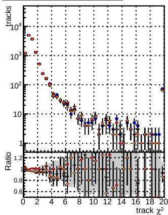
N of reco track vs. \chi^2 for BSM mFit, TFit, TFit+WS, genMatch-CUT2, BSM mFit, TFit, TFit+WS, genMatch-CUT2
