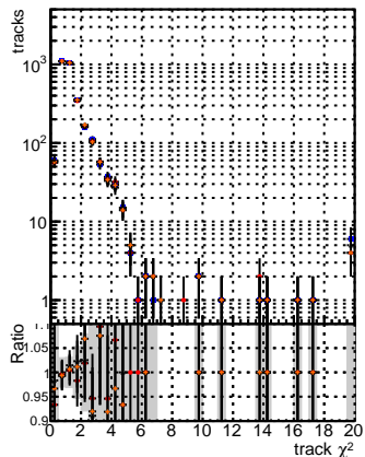
N of reco track vs. \chi^2 BGM mFit TFit TFit+WS genMatch-CUT2 BGM+mFit BGM+TFit BGM+mFit+TFit+WS+genMatch-CUT2
