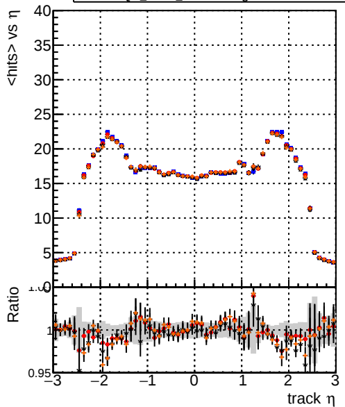
DQM_mkFit_TToriginal DQM_mkFit_TTNEWnoMS-genMatch-CUT2 DQM_mkFit_TToriginal-106 DQM_mkFit_TTNEWMS-genMatch-CUT2 mean hit
