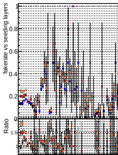
Fake rate vs. DQM mkFit TtoOriginal TtoWMS-genMatch-CUT2 DQM mkFit TtoWMS-genMatch-CUT2
