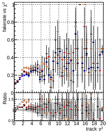
Fake rate vs. DQM mkFit TtoOriginal TtoWMS-genMatch-CUT2 DQM mkFit TtoWMS-genMatch-CUT2
