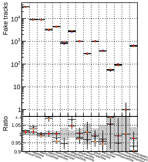
Number Legend 1 DQM_mkFit_TTNEWMS-genMatch-CUT2 2 DQM_mkFit_TToriginal-106 3 DQM_mkFit_TTNEWMS-genMatch-CUT2
