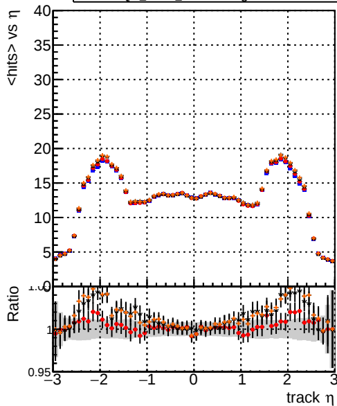
Legend: DQM_mkFit_TToriginal (blue line), DQM_mkFit_TTNEWnoMS-genMatch-CUT2 (red line), DQM_mkFit_TTOriginal-106 (black line), DQM_mkFit_TTNEWMS-genMatch-CUT2 (orange line) mean hit
