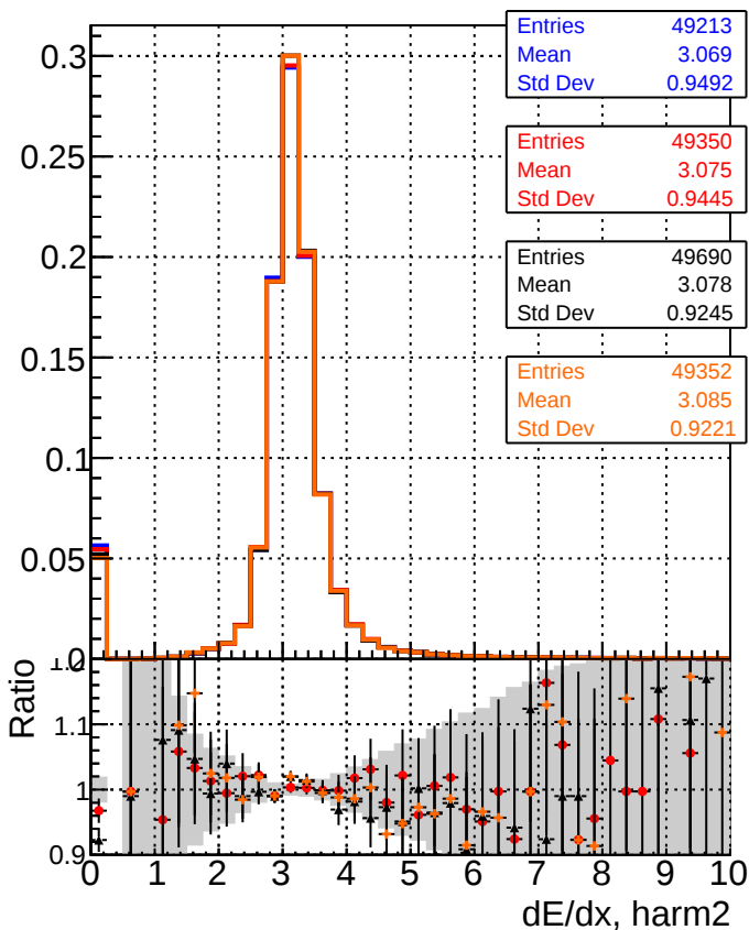
— DQM_mkFit_TToriginal — DQM_mkFit_TTNEWnoMS-genMatch-CUT2 — DQM_mkFit_TToriginal-106 — DQM_mkFit_TTNEWMS-genMatch-CUT2
