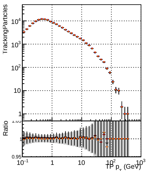
—•— DQM_mkFit_TToriginal —•— DQM_mkFit_TTNEWnoMS-genMatch-CUT2 —•— DQM_mkFit_TToriginal-106 —•— DQM_mkFit_TTNEWMS-genMatch-CUT2
