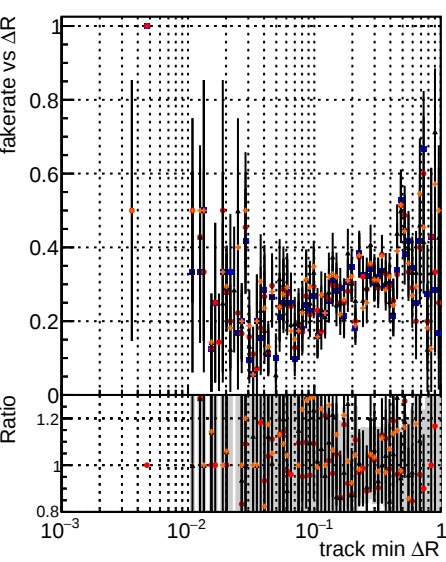
Fake rate vs \Delta R(\text{track, jet}) for MS-genMatch-CUT2, Whim-100, and NEWS-genMatch-CUT2 methods.
