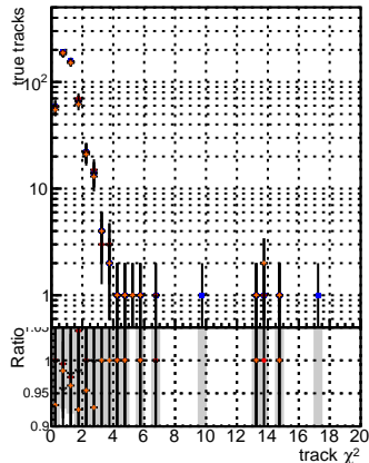
N of reco track vs. \chi^2 for BGM, mFit, True, WMS, genMatch-CUT2, mFit, True, WMS, genMatch-CUT2
