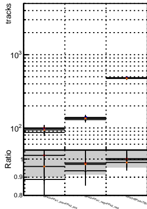
N of reco track vs. \chi^2 for BGM, mFit, True, WMS, genMatch-CUT2, mFit, True, WMS, genMatch-CUT2
