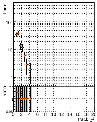
N of reco track vs. \chi^2 BSM mFit TrueWMS genMatch-CUT2 BSM mFit TrueWMS genMatch-CUT2 BSM mFit TrueWMS genMatch-CUT2
