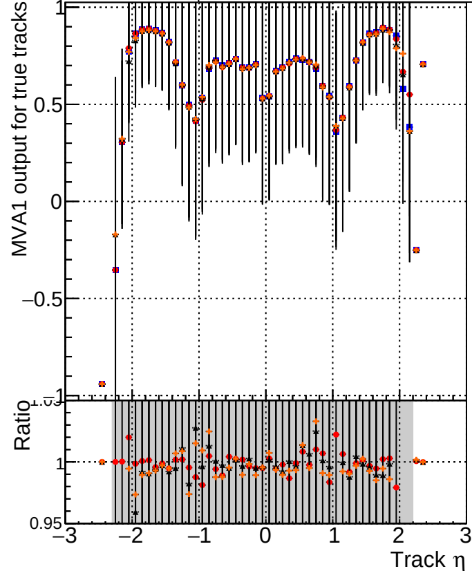
MVA1 of associated tracks (recoToSim) vs. track \eta Legend: DQM_mkFit_TToriginal (blue square) DQM_mkFit_TTNEWnoMS-genMatch-CUT2 (red circle) DQM_mkFit_TToriginal-106 (black triangle) DQM_mkFit_TTNEWMS-genMatch-CUT2 (orange diamond)
