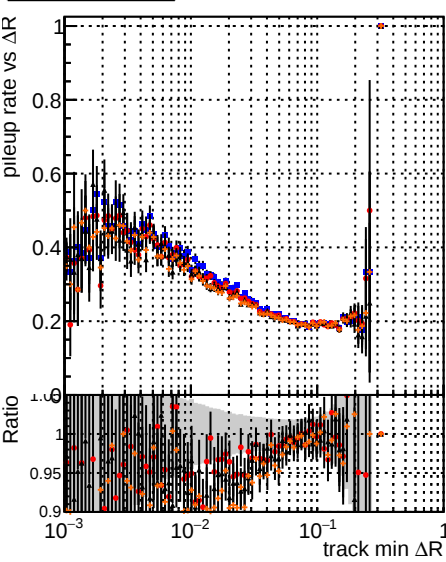
DOM mkFit T-Original DOM mkFit T-Original MS-genMatch-CUT2 DOM mkFit T-Original MS-genMatch-CUT2 DOM mkFit T-Original MS-genMatch-CUT2
