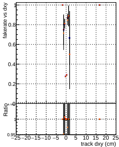
Legend for all plots: DOM mktFit TToriginal DOM mktFit TTWMS-genMatch-CUT2 DOM mktFit TTWMS-genMatch-CUT2
