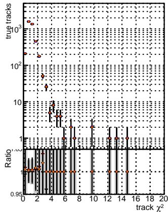
N of reco track vs. \chi^2 for BGM, mFit, True, genMatch-CUT2, mFit, True, genMatch-CUT2, mFit, True, genMatch-CUT2
