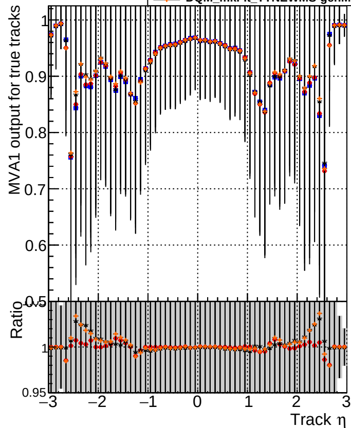
MVA1 of associated tracks (recoToSim) vs. track \eta Legend: \blacksquare DQM_mkFit_TToriginal \bullet DQM_mkFit_TTNEWnoMS-genMatch-CUT2 \blacktriangledown DQM_mkFit_TToriginal-106 \blacklozenge DQM_mkFit_TTNEWMS-genMatch-CUT2
