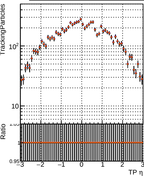
◆ DQM_mkFit_TToriginal ◆ DQM_mkFit_TTNEWnoMS-genMatch-CUT2 ◆ DQM_mkFit_TToriginal-106 ◆ DQM_mkFit_TTNEWMS-genMatch-CUT2
