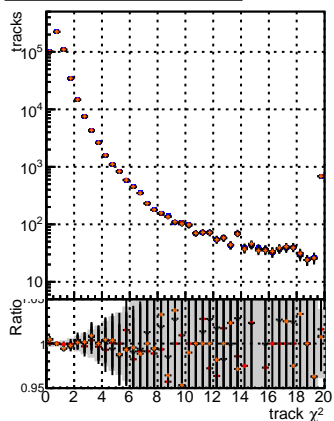
N of reco track vs. \chi^2 for BGM, mFit, and Original tracks. The legend indicates the track type: BGM (blue), mFit (orange), and Original (red). The x-axis is track \chi^2 and the y-axis is the number of tracks.
