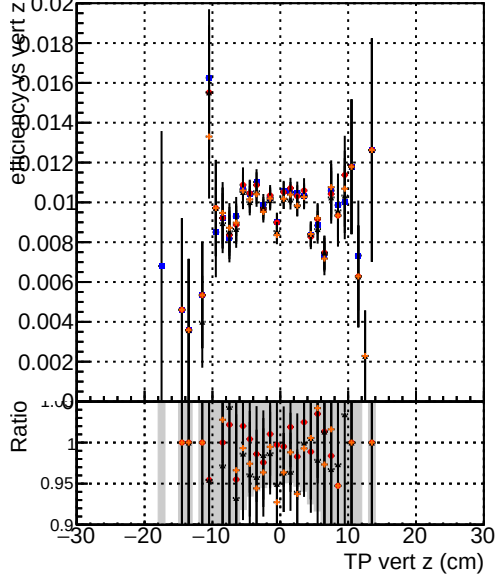
Efficiency vs TP vert z —●— DQM_mkFit_TToriginal —●— DQM_mkFit_TTNEWnoMS-genMatch-CUT2 —●— DQM_mkFit_TToriginal-106 —●— DQM_mkFit_TTNEWMS-genMatch-CUT2
