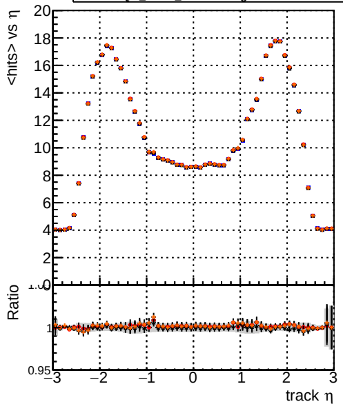
mean hit DOM_mkFit_TToriginal DOM_mkFit_TTNEWnoMS-genMatch-CUT2 DOM_mkFit_TToriginal-106 DOM_mkFit_TTNEWMS-genMatch-CUT2
