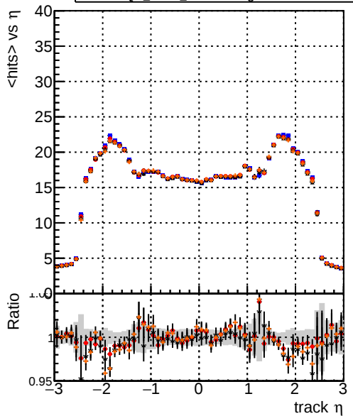
Legend: DQM_mkFit_TToriginal (blue line), DQM_mkFit_TTNEWnoMS-genMatch-CUT2 (red line), DQM_mkFit_TTOriginal-106 (black line), DQM_mkFit_TTNEWMS-genMatch-CUT2 (orange line) mean hit
